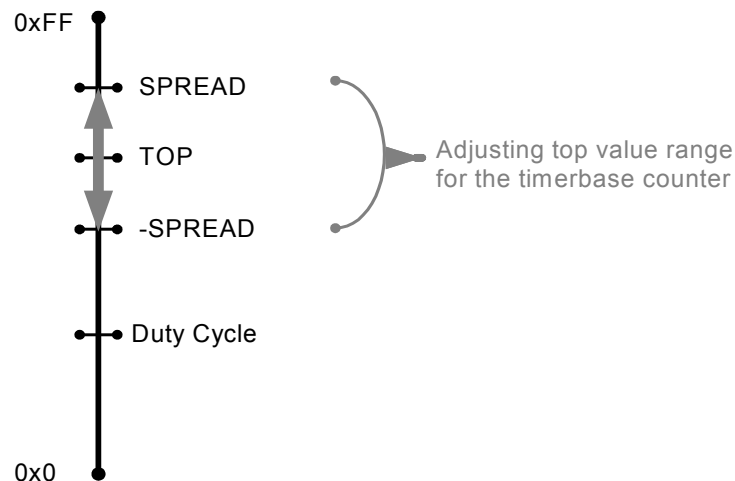
Figure 23-2. PWMA Adjusting Top Value for Timebase Counter
