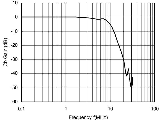
Cb System Filter Characteristics (Vcc=4.8V)
