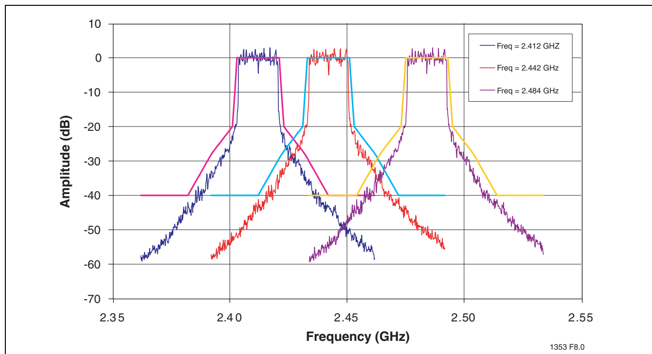
FIGURE 8: 802.11g Spectrum Mask at 23 dBm
