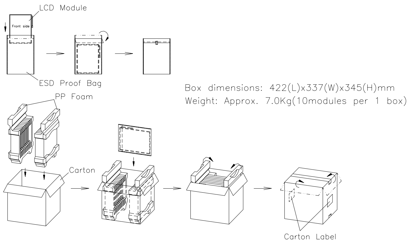
Figure. 7-1 Packing method
