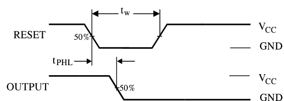
Figure 2. Switching Waveforms
