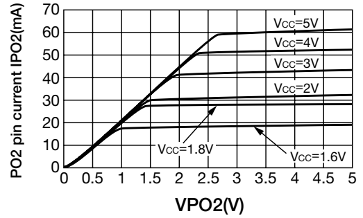
PO2 pin current characteristics
