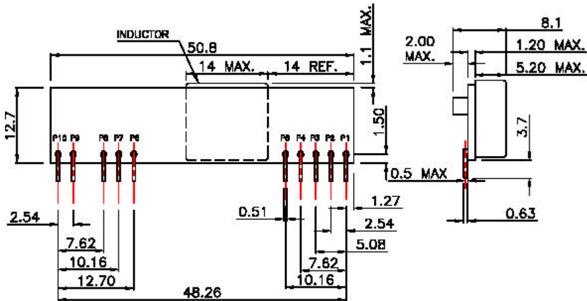
Mechanical Dimensions - Vertical type
