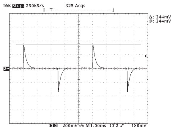
Figure 11 - RFF600-24S28Y Transient Response Load 10.70 A to 16.05 A
