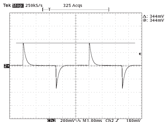
Figure 11 - RFF600-24S28Y Transient Response Load 10.70 A to 16.05 A
