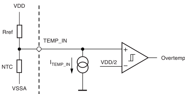
Figure 7-2. Overtemperature Detection
