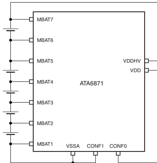
Figure 7-4. 5 Cells Operation
