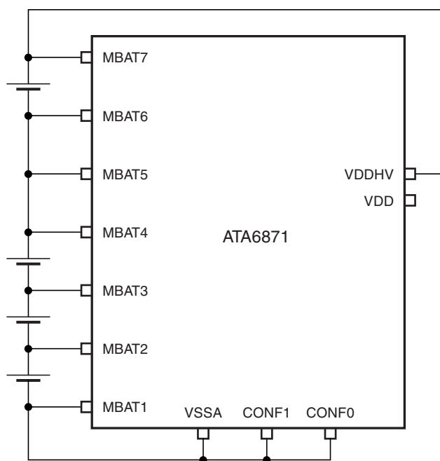
Figure 7-5. 4 Cells Operation
