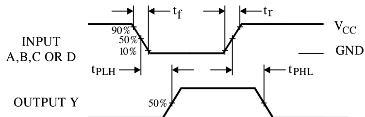
Figure 1. Switching Waveforms
