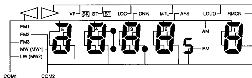
Figure 2. LCD-8162JP common pattern
