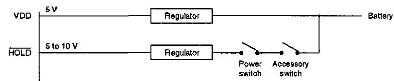
Figure 24. Power supply switch configuration
