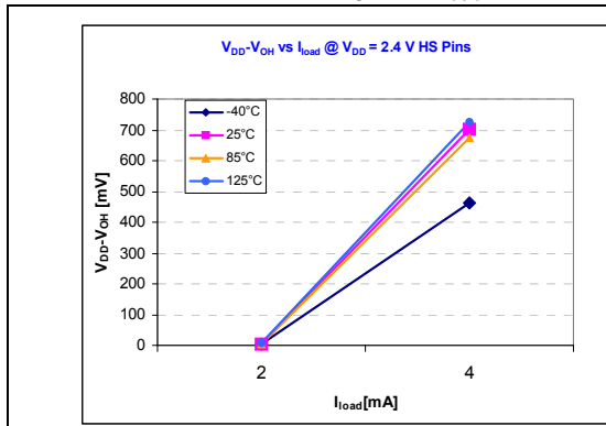
Figure 17. Typical V_{DD}-V_{OH} vs. I_{load} at V_{DD} = 2.4\text{ V}
