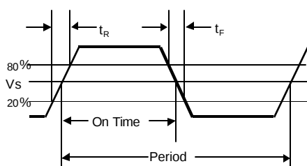
Figure 1. Output Waveform
