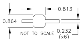
DETAIL OF LEADS # 3, 5, 11, 17, 19 & 25
