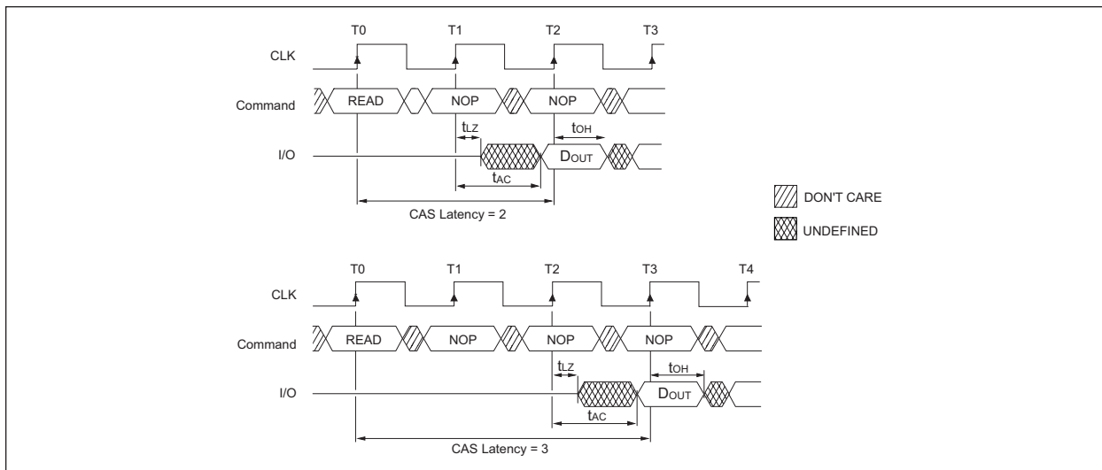
FIGURE 4 – CAS LATENCY
