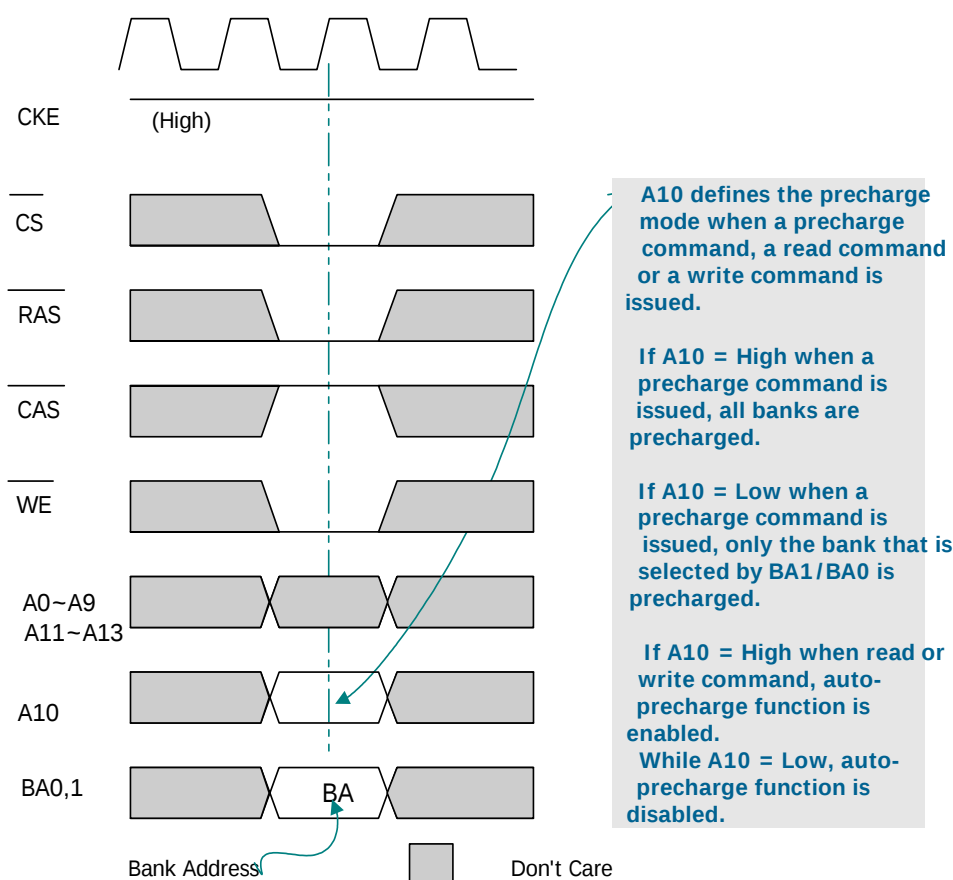
PRECHARGE command
