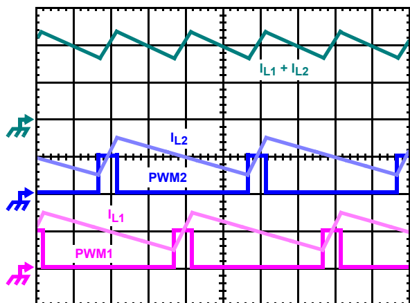
FIGURE 2. PWM AND INDUCTOR-CURRENT WAVEFORMS FOR 2-PHASE CONVERTER
