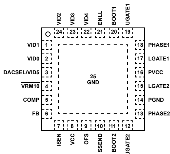
ISL6563 (QFN) TOP VIEW
