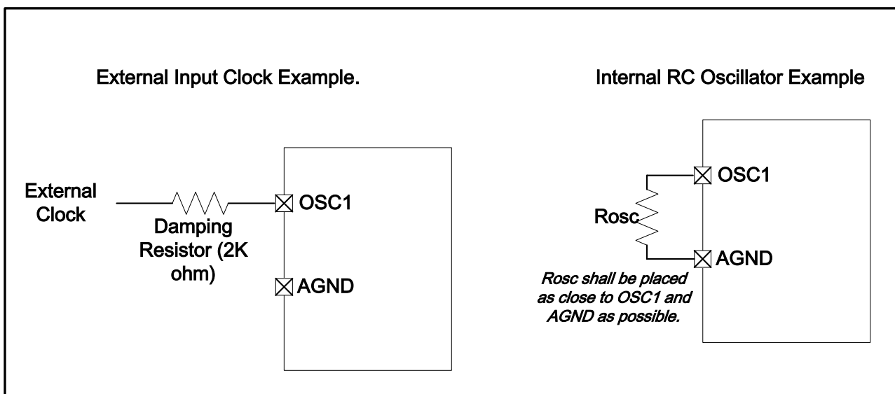
Figure 46 Oscillation Connection
