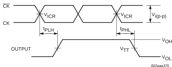
Fig 9. Voltage waveforms; propagation delay times.
