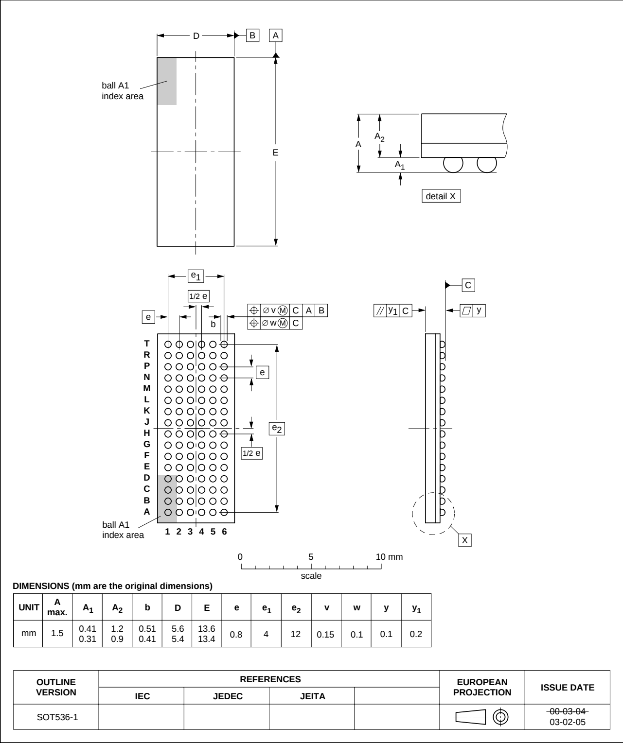
Fig 15. LFBGA96 package outline (SOT536-1).
