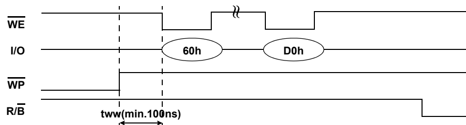
Figure C-2. Erase Operation
