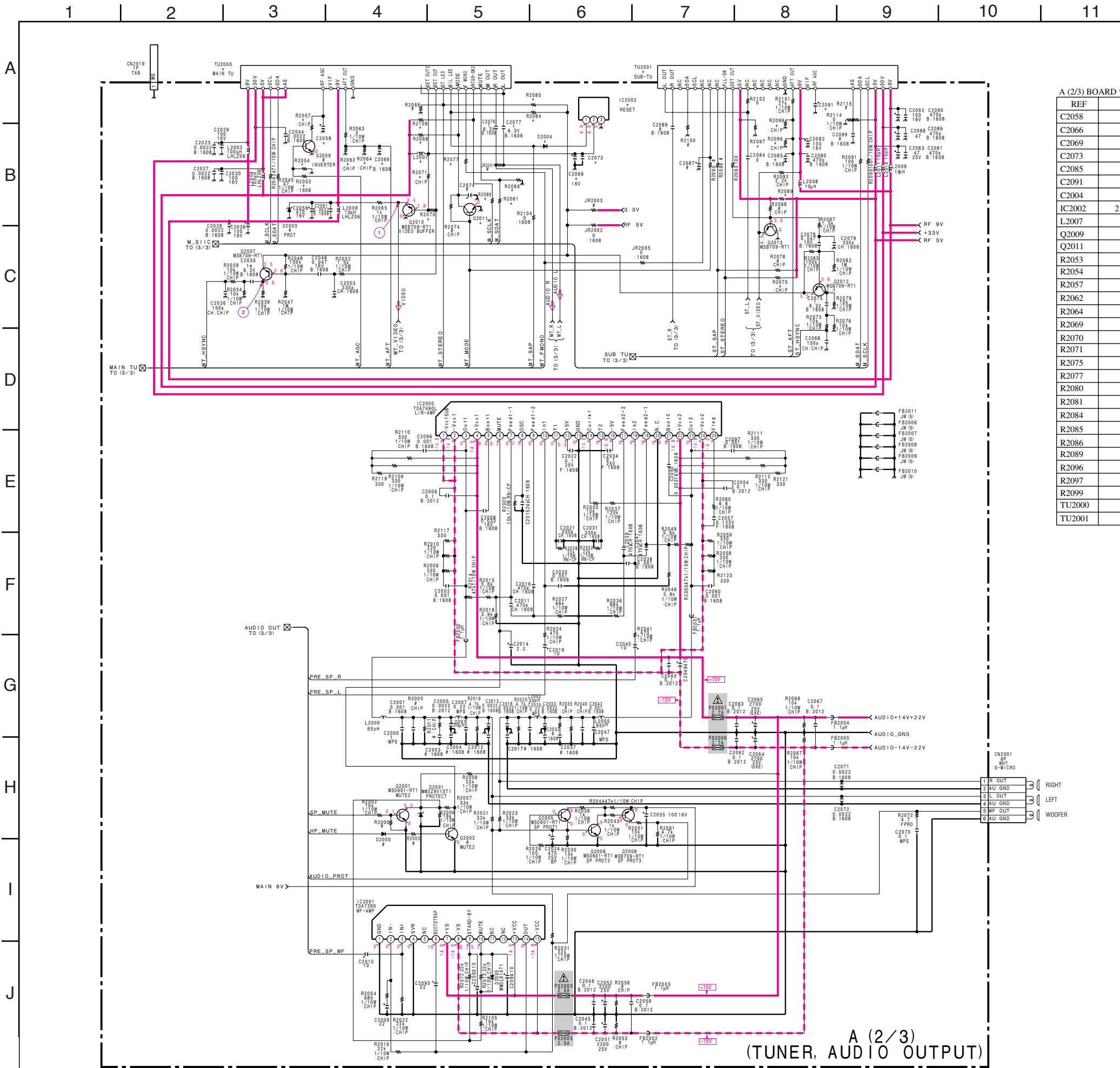
(2) Schematic Diagram of A (2/3) Board
