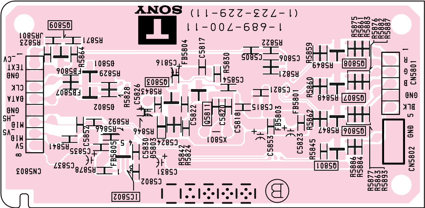
— T BOARD (B Side) —
