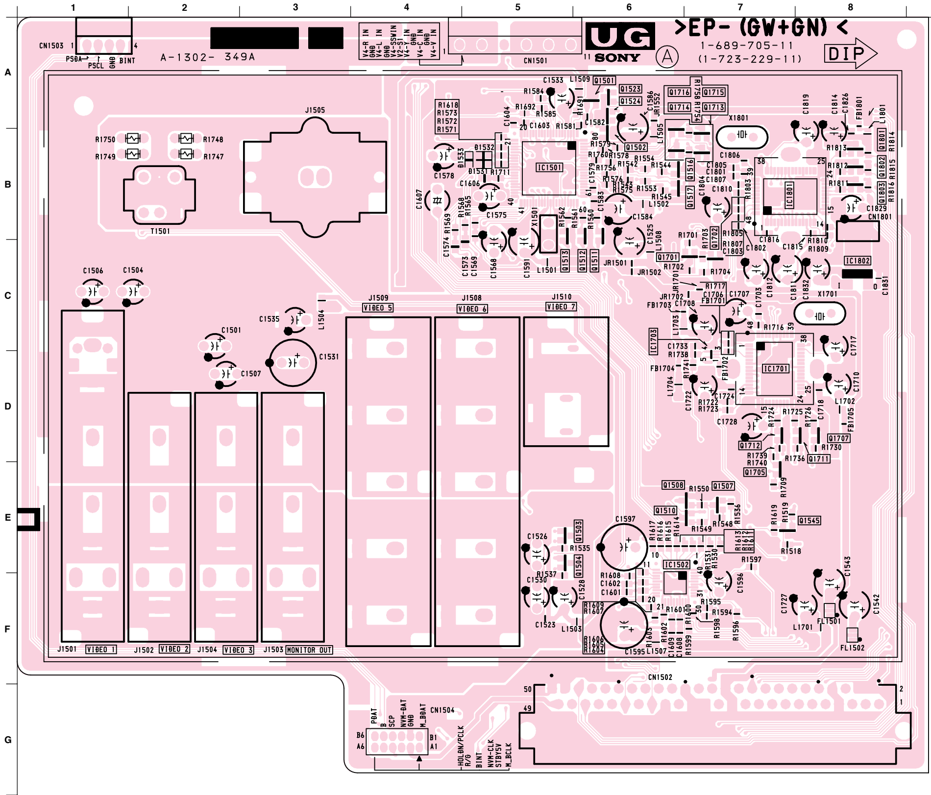
— UG BOARD (A Side) —
