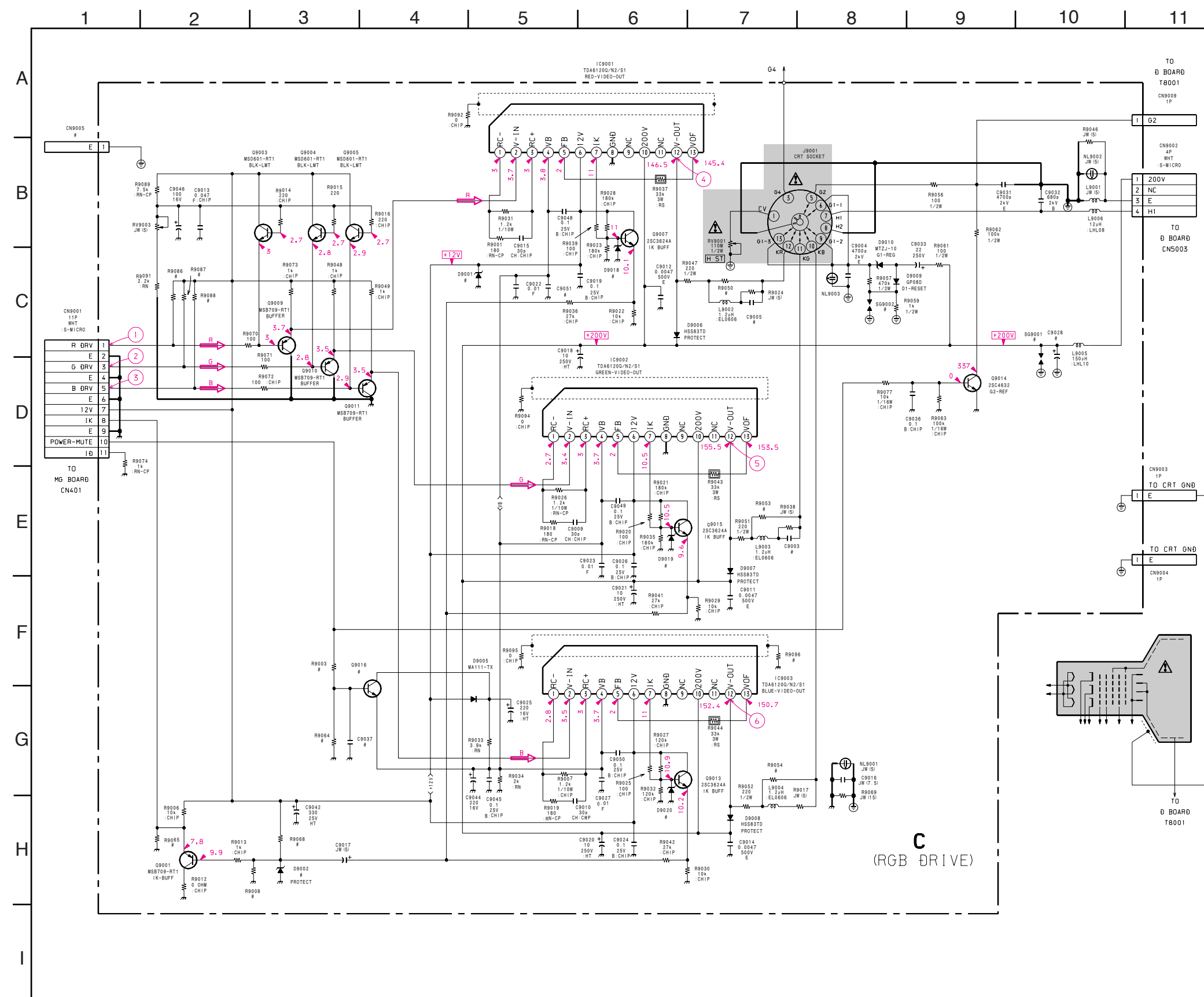
(8) Schematic Diagram of C Board
