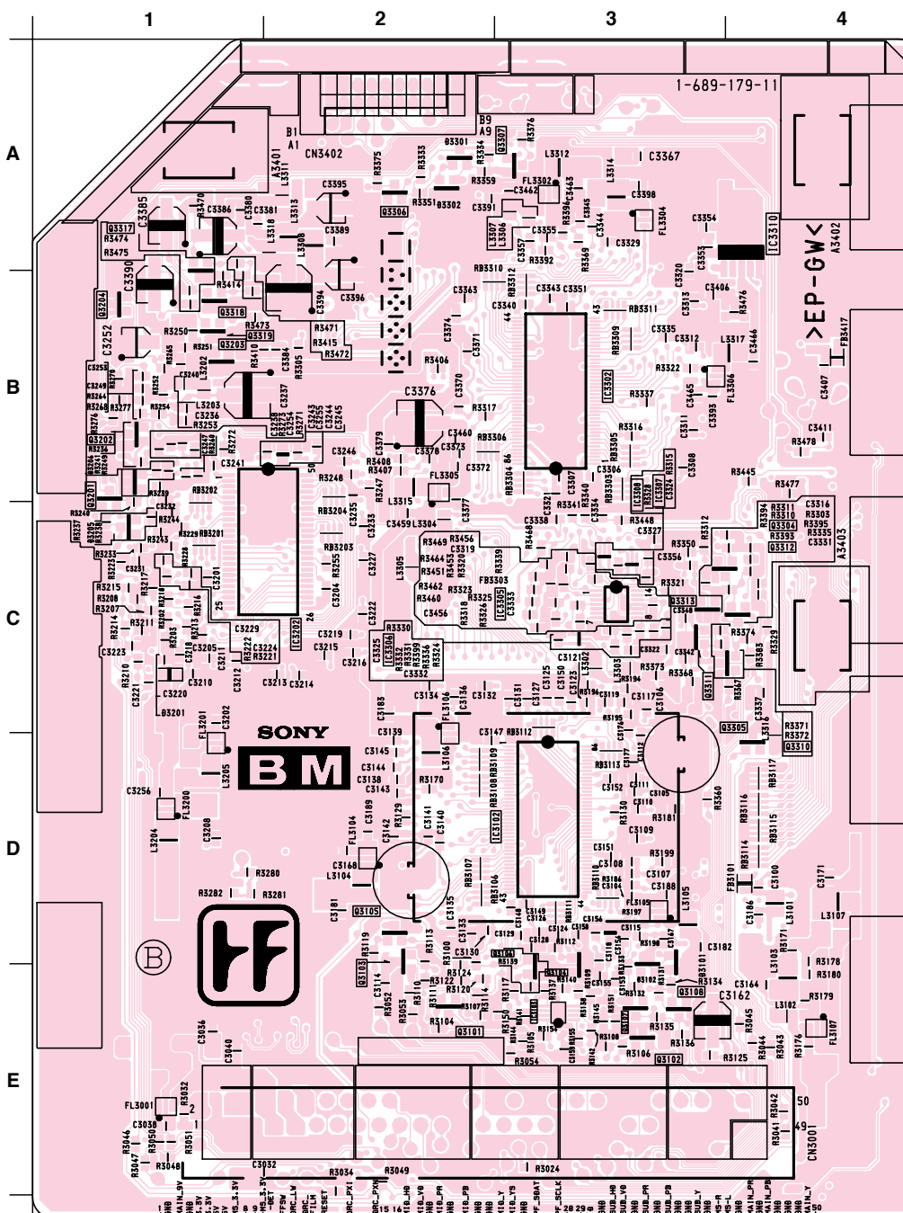
— BM BOARD (B Side) —
