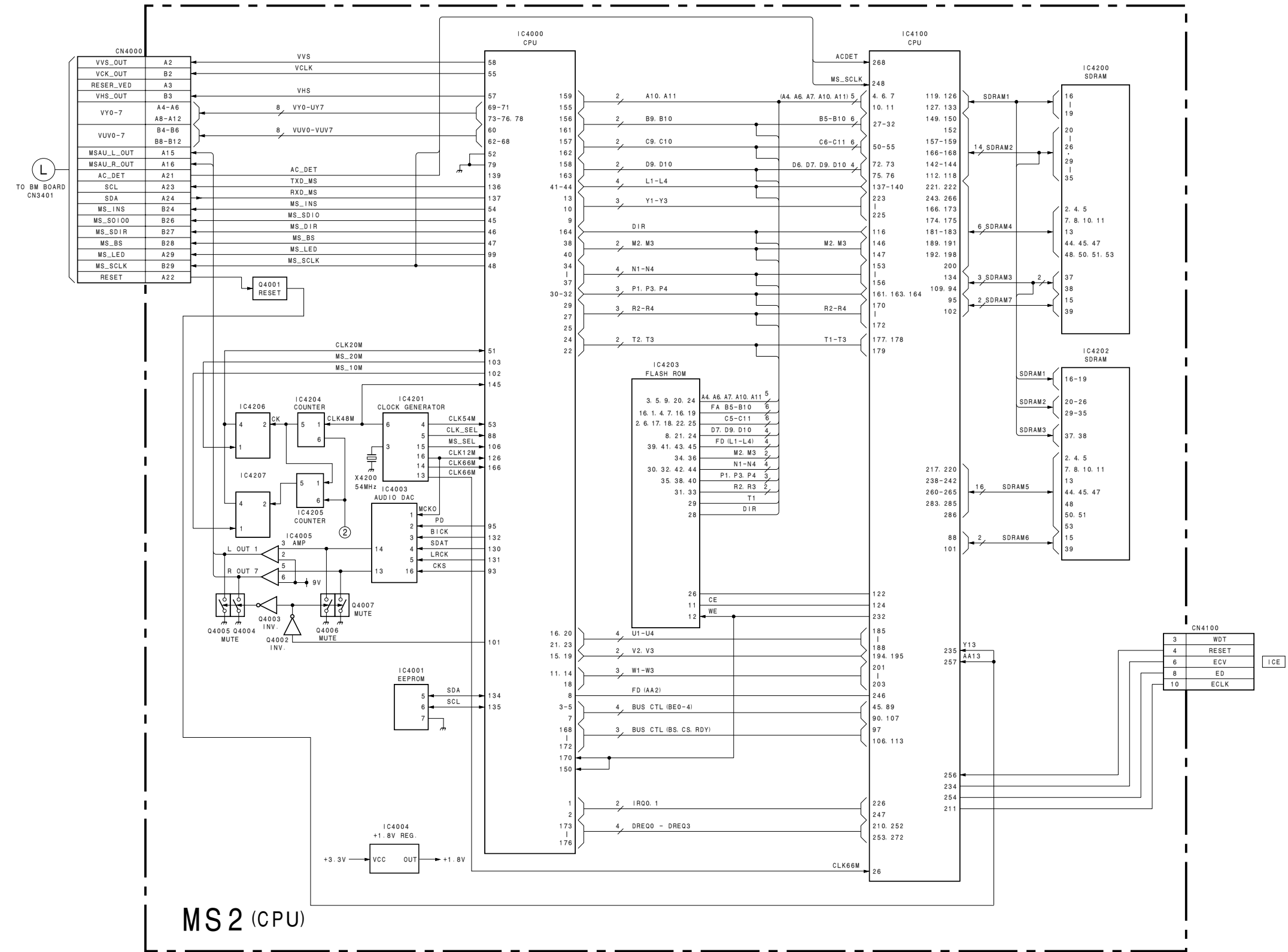
BLOCK DIAGRAM (6)
