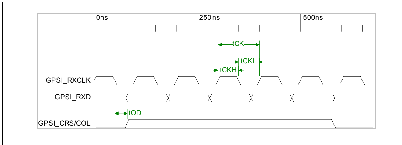
Figure 12 GPSI (7-wire) Input Timing
