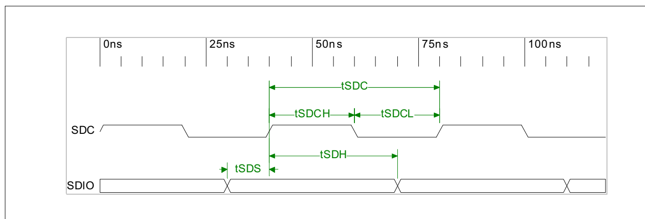
Figure 15 SMI Timing
