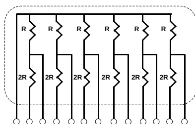
Fig. 4: LADDER CIRCUIT
