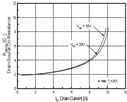
Fig.3 On-Resistance Variation vs Drain Current
