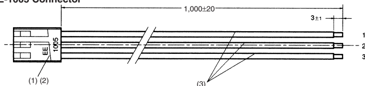
EE-1005 Connector
