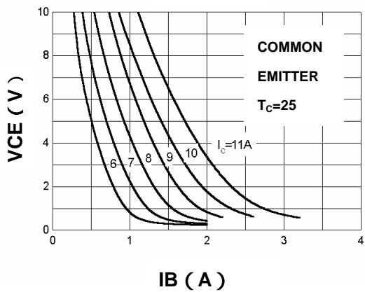
VCE - IB
