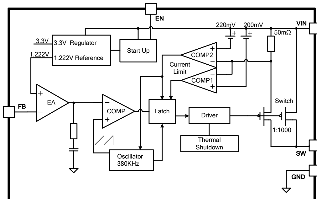
Figure3. Function Block Diagram of XL1410
