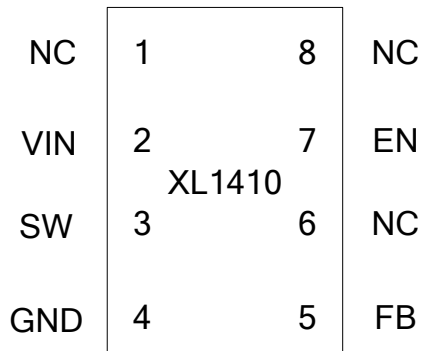
Figure2. Pin Configuration of XL1410 (Top View)
