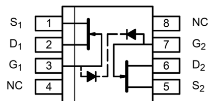
SOIC (Top View)
