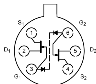
TO-71 (Top View)
