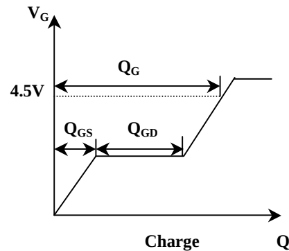
Fig 12. Gate Charge Waveform
