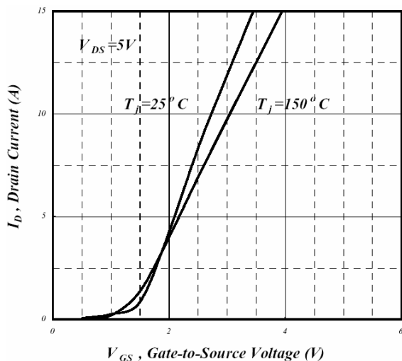
Fig 11. Transfer Characteristics
