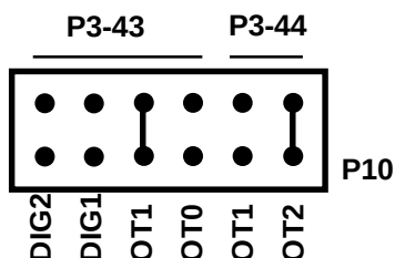
Fig. 1-2 — P3 Signal Select Jumpers, P10
