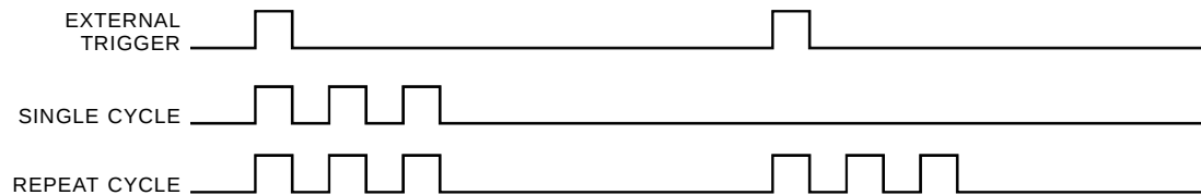
Fig. 5-4 — External Trigger Single Cycle Vs. Repeat Cycle
