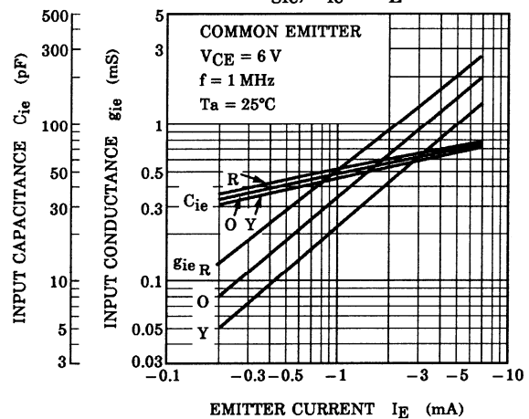
g_{ie}, C_{ie} - I_E
