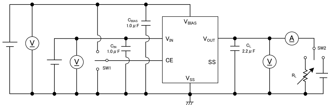
CIRCUIT①
