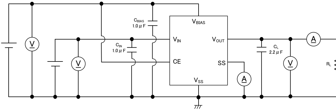
CIRCUIT⑤
