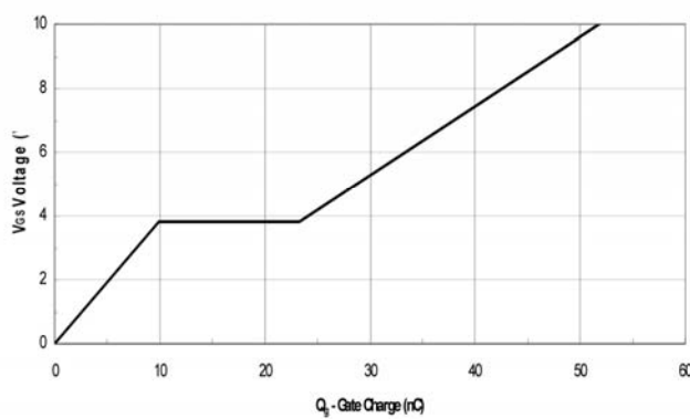
Gate Charge
