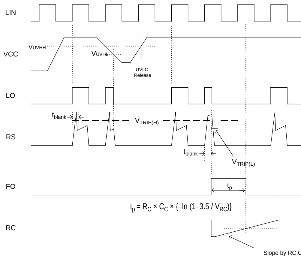
Low Side Driver Input/Output Timing Diagrams
