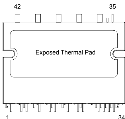
Pin-out Diagram
