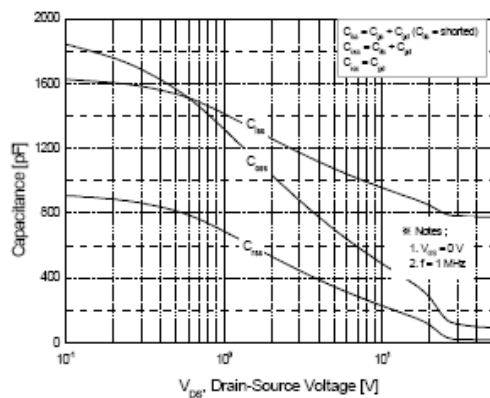
Fig.5 Capacitance Characteristics
