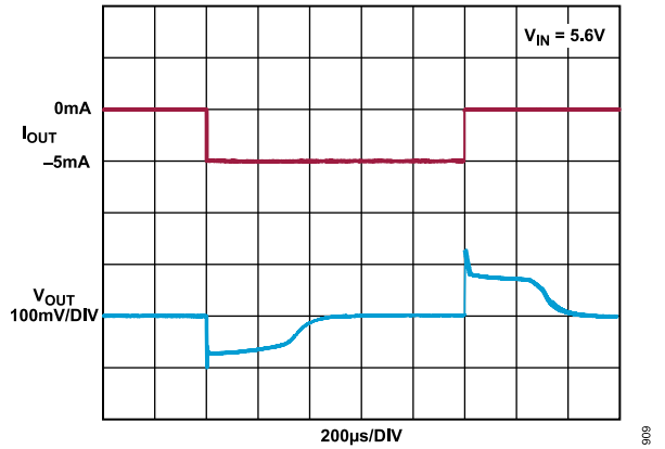
Figure 85. ADR4540 D Grade Load Transient Response (Sourcing)
