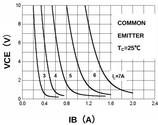
VCE - IB
