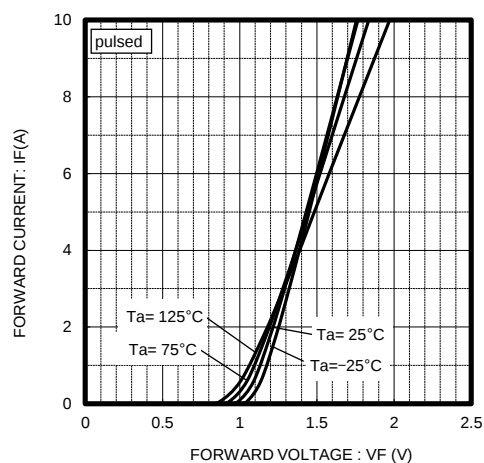
Fig.2 VF-IF Characteristics
