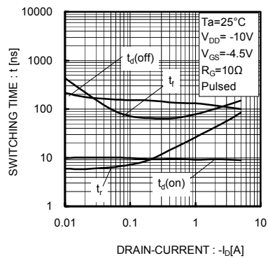
Fig.14 Switching Characteristics
