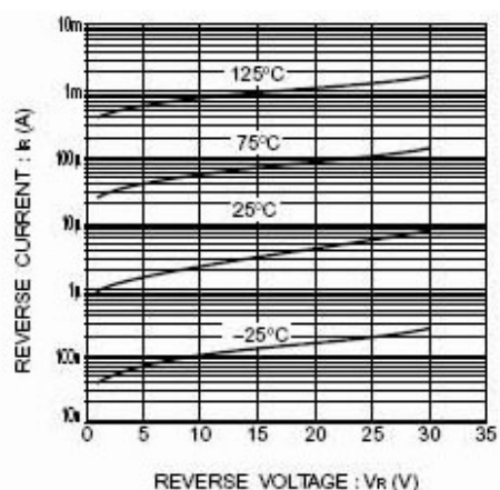
Fig.2 Reverse characteristics
