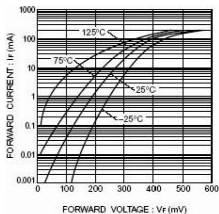
Fig.1 Forward characteristics
