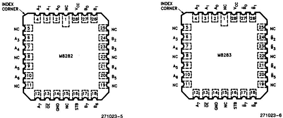
Figure 2. Pin Configurations
