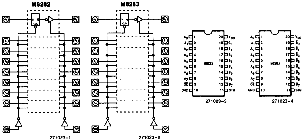
Figure 1. Logic Diagrams
