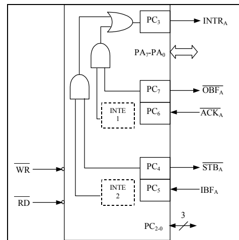
Figure 14. MODE 2
