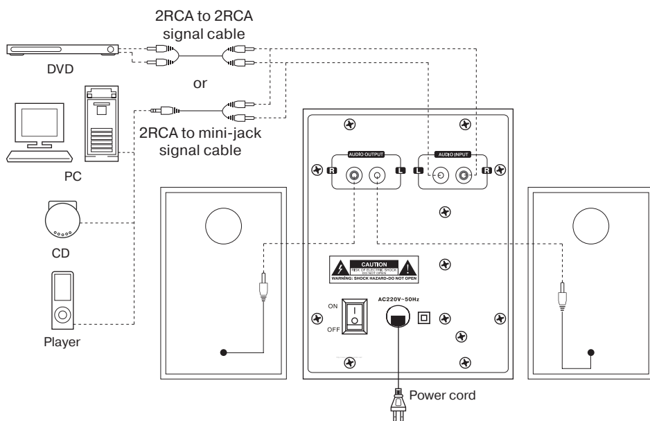
Fig. 3. Connection diagram
