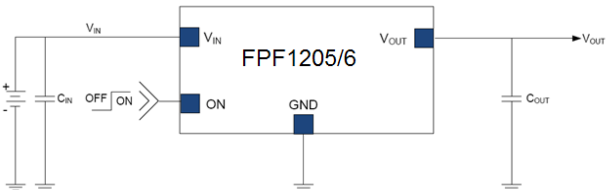
Figure 1. Typical Application
