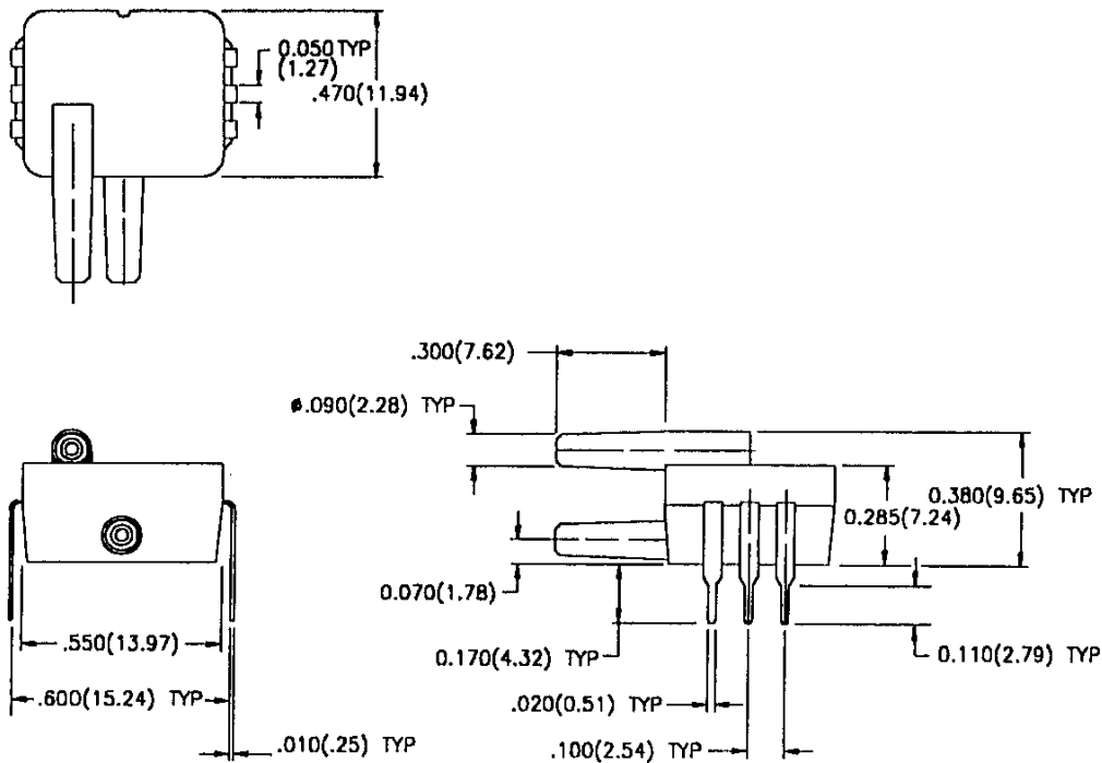
Basic Sensor DIP "D4" Package
