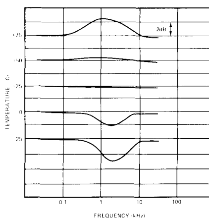
FIGURE 12 BACK-TO-BACK FREQUENCY RESPONSE VERSUS TEMPERATURE ENCODE AT +25°C AND -20dB
