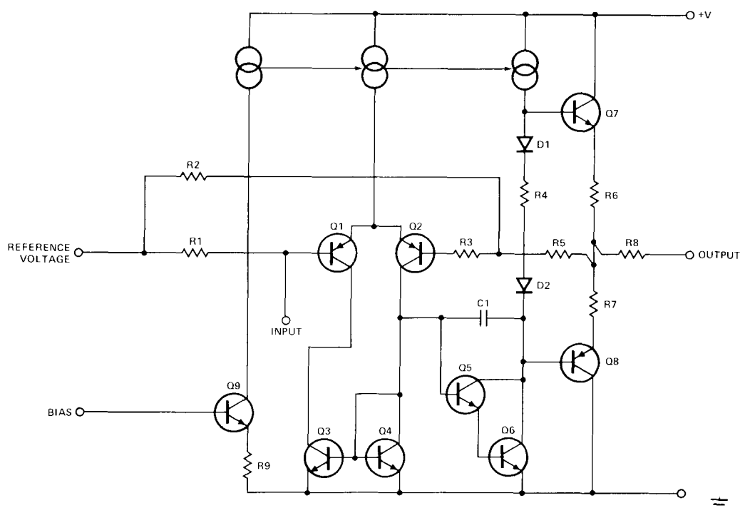
FIGURE 26 BASIC OPERATIONAL AMPLIFIER
