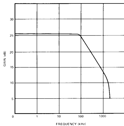
FIGURE 5 VOLTAGE GAIN PIN 5 TO PIN 3
