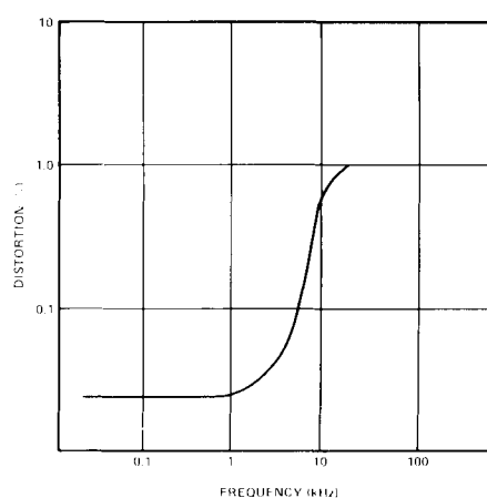
FIGURE 8 DISTORTION VERSUS FREQUENCY 0dB DECODE
